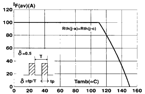
Fig.6 : Average current versus ambient temperature. (duty cycle : 0.5)
